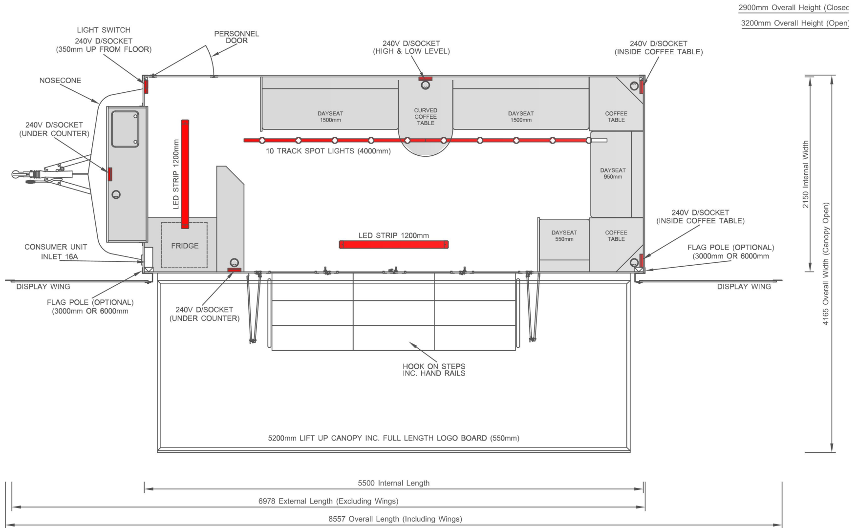
Plan view with lights and electrical sockets highlighted
