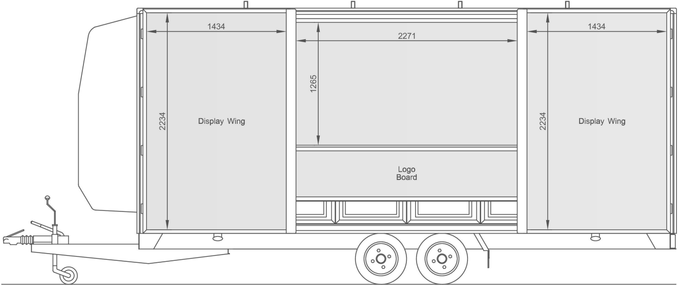
NEAR SIDE VIEW (CLOSED)
