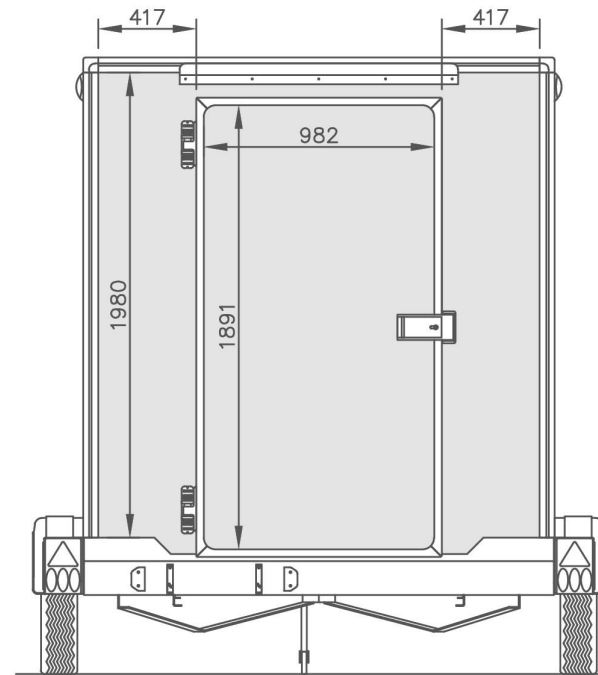
REAR VIEW
